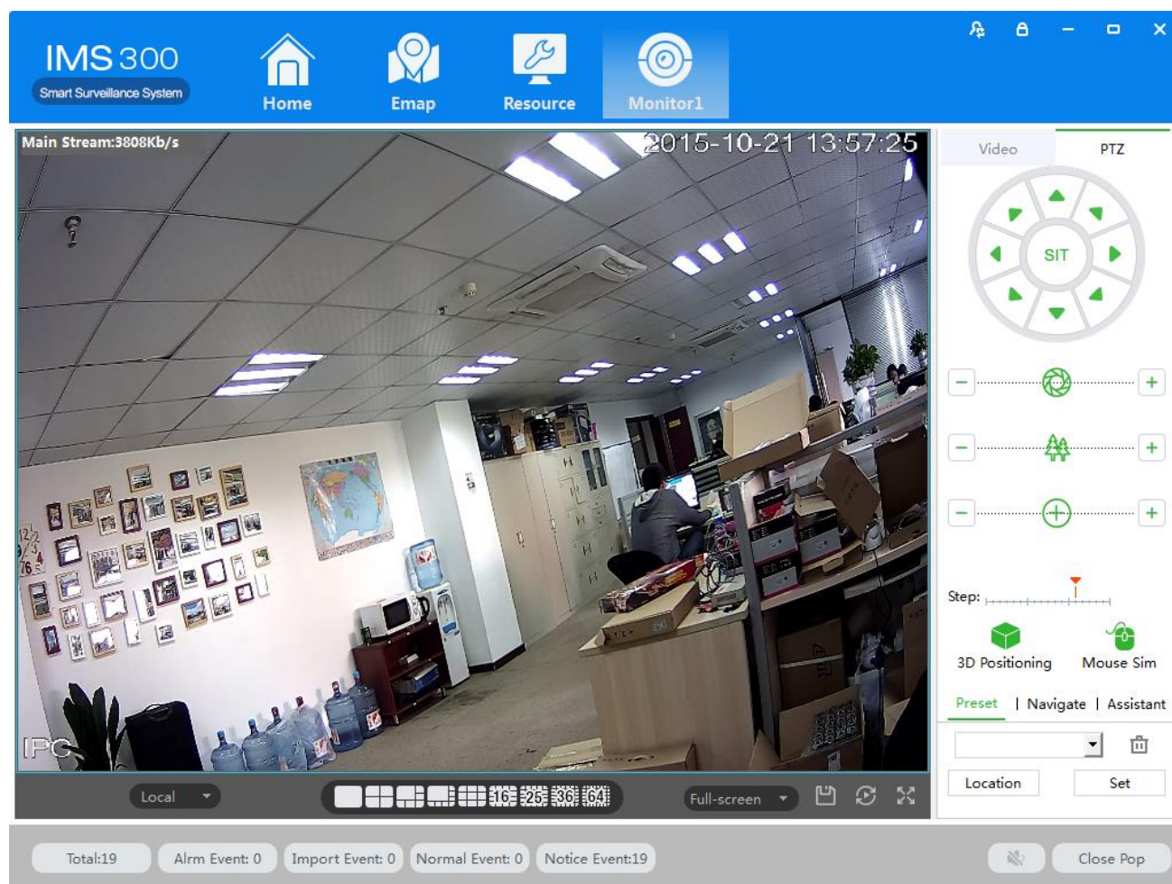
Figure 4-3 PTZ control
