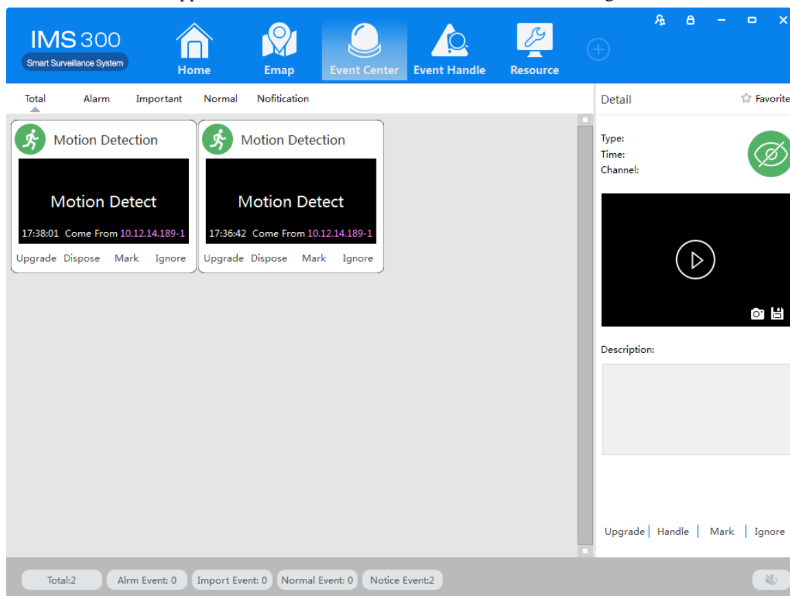
Figure 7-1 Event Center
