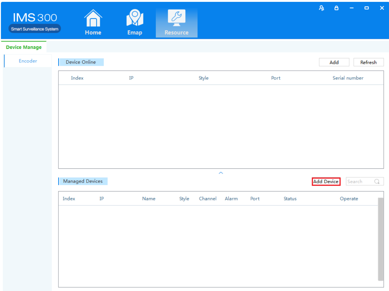
Figure 3-3 Resource Management
