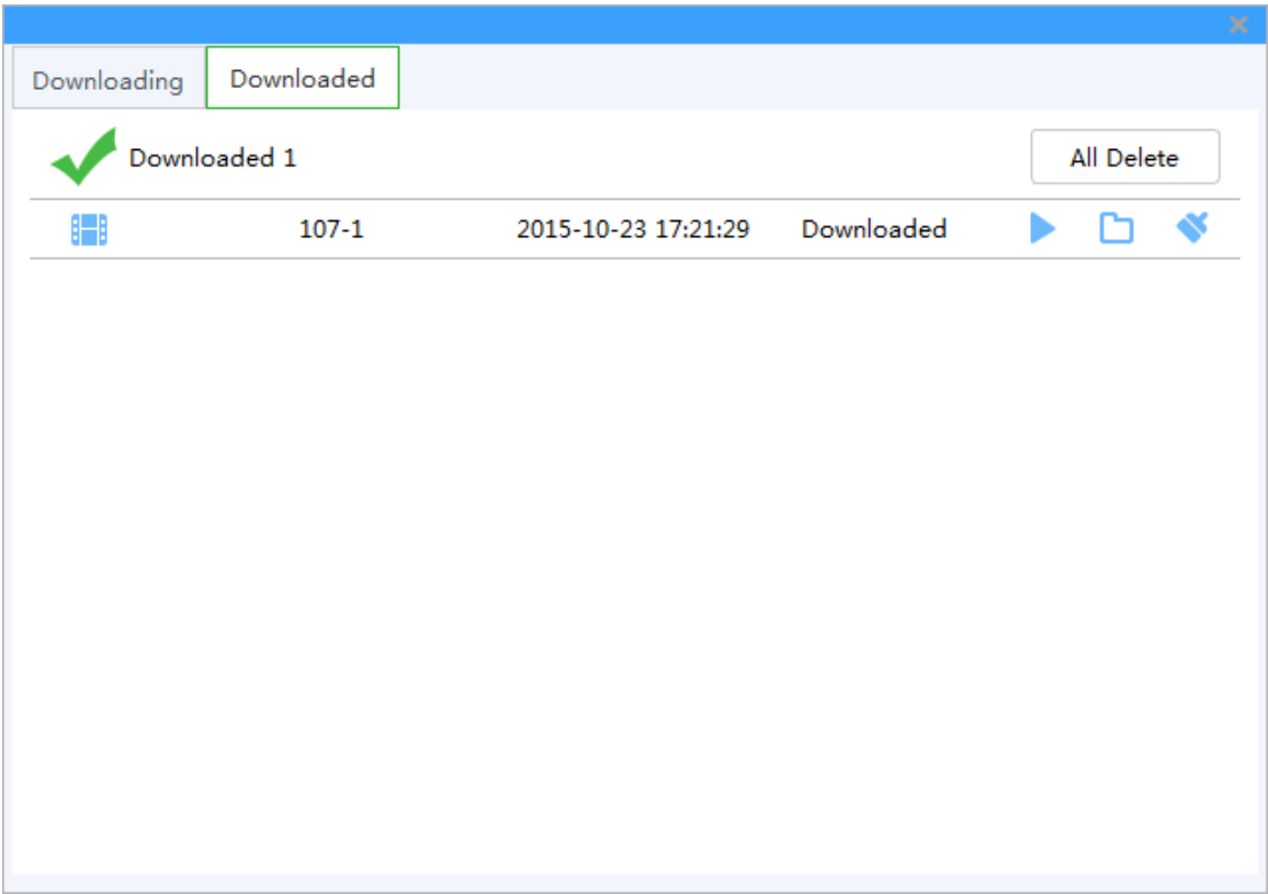
Figure 4-6 Finished list
