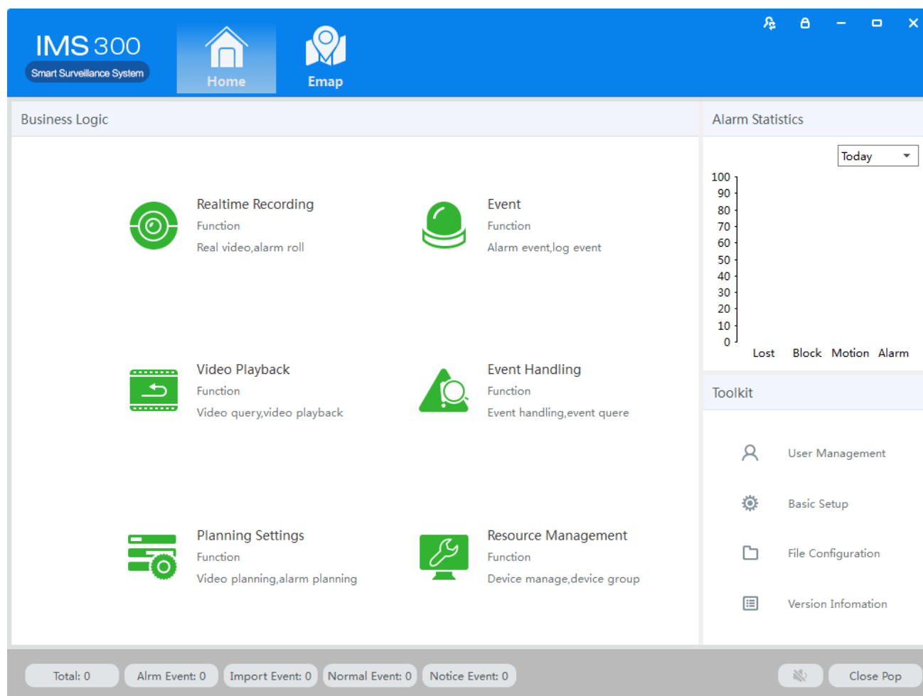
Figure 3-2 Clients homepage
