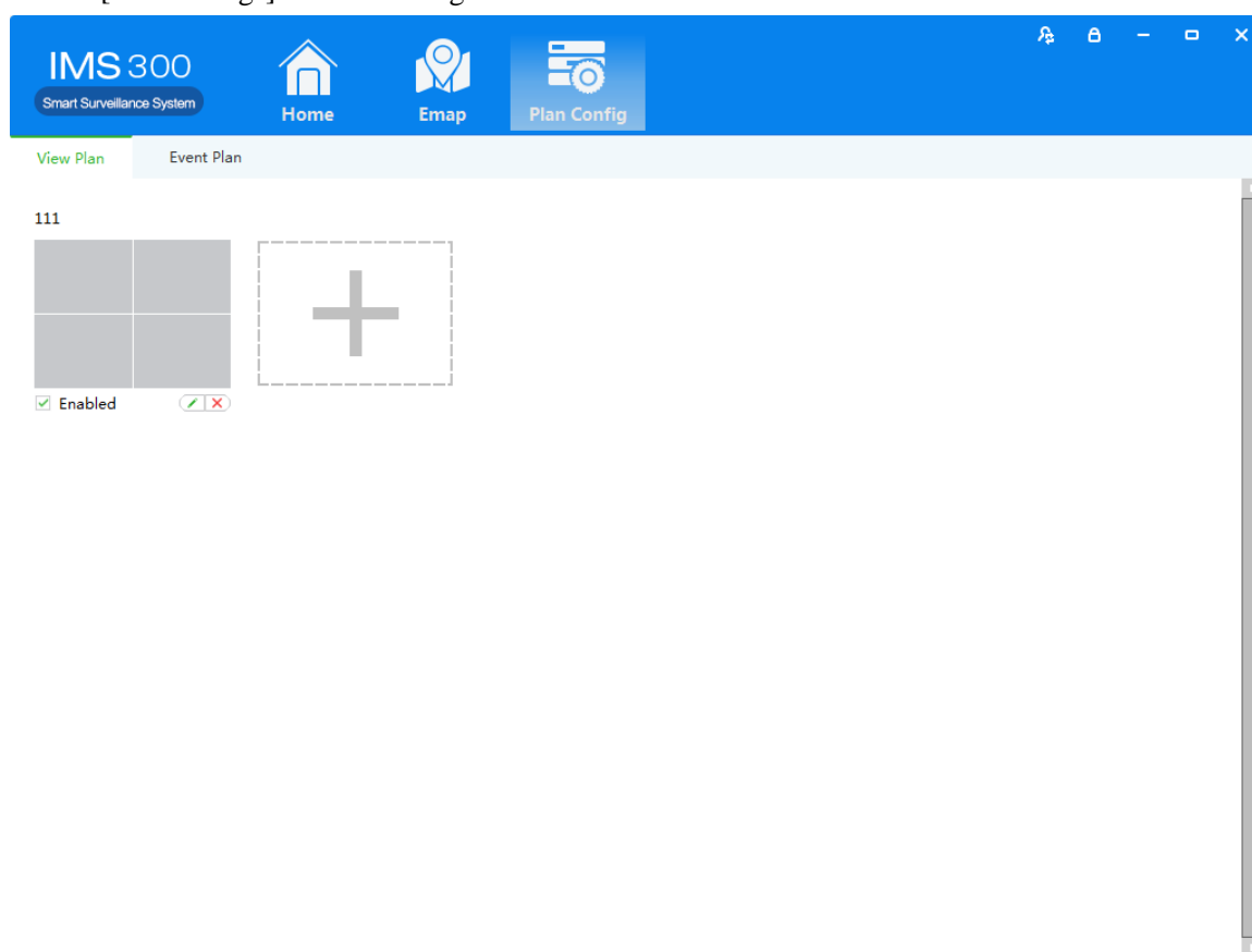
Figure 8-3 Plan settings
