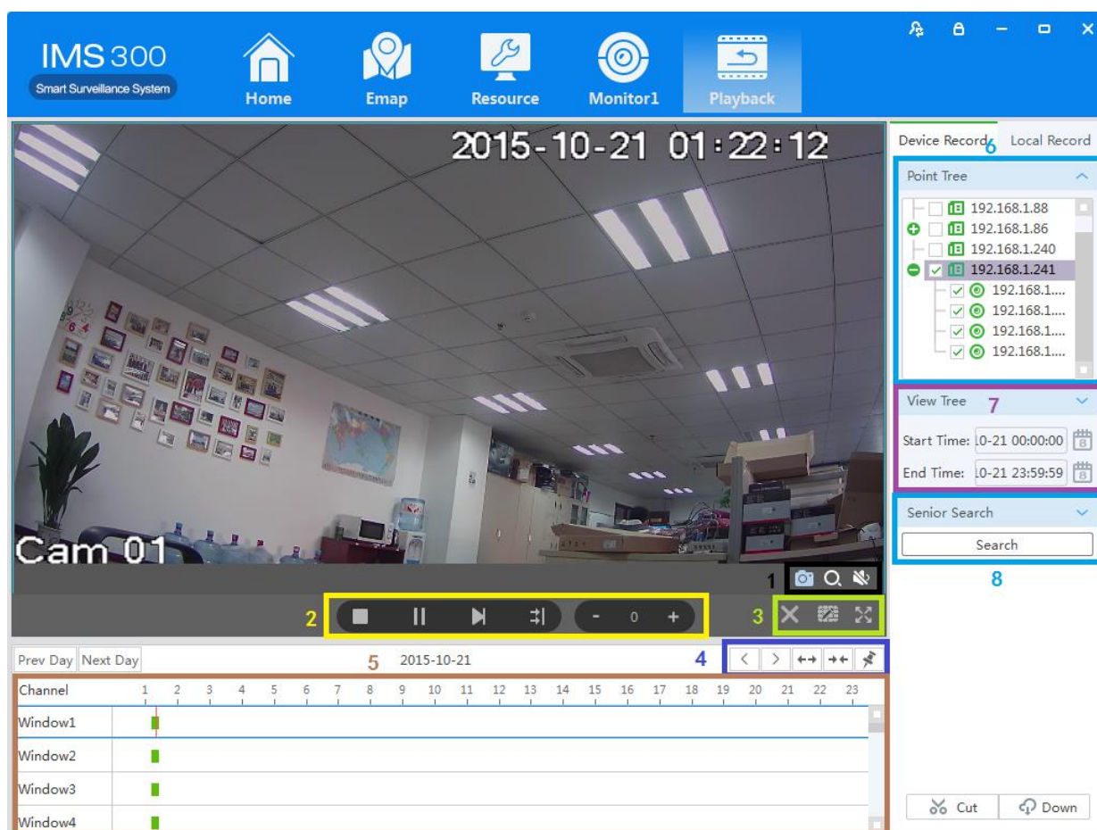
Figure 5-1 Video playback
