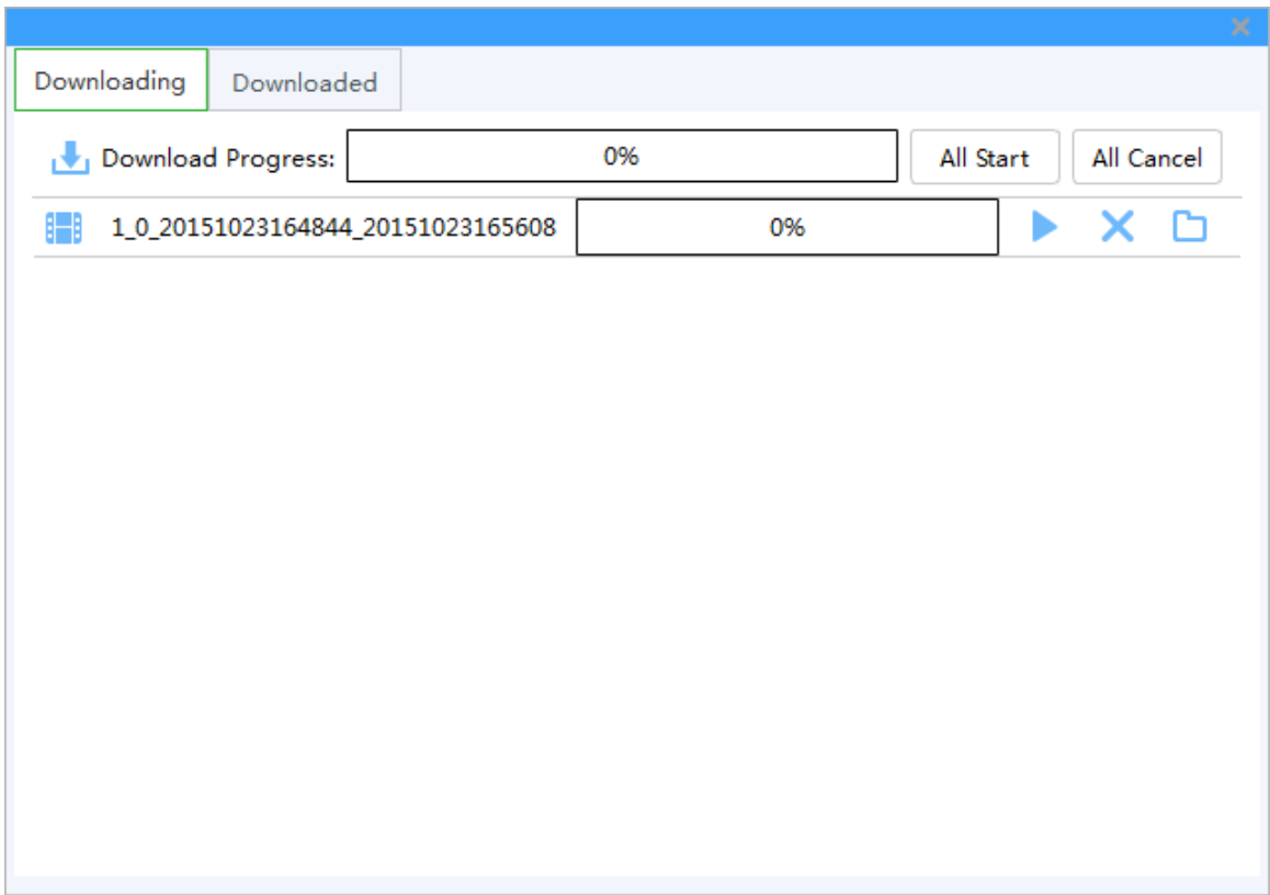
Figure 4-5 Video download
